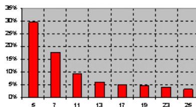
Harmonic disturbance with and without AHF filter.
